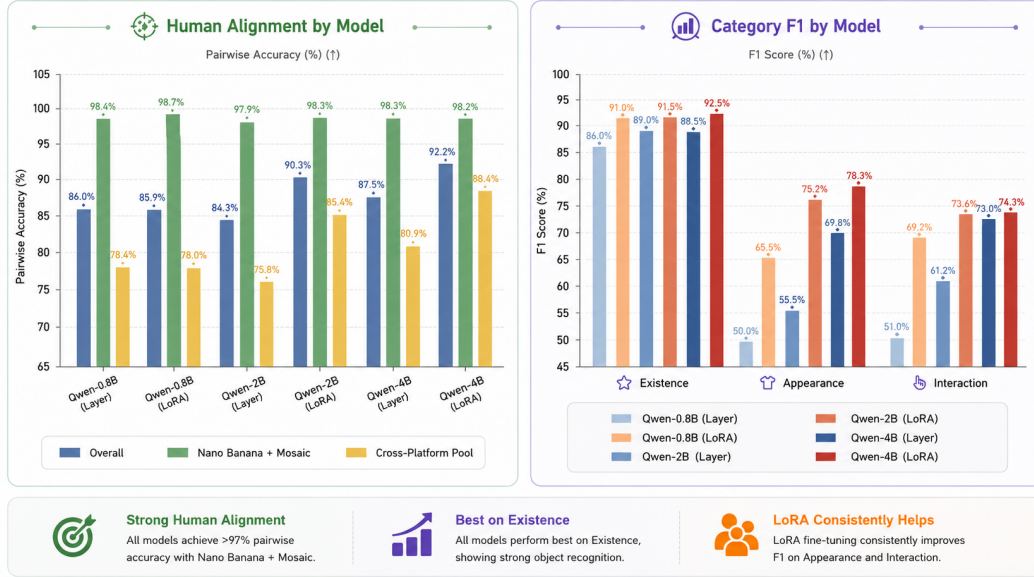
Figure 4: Human alignment of MIE variants on MIB-GoId. Left: overall, seen-generator, and unseen-generator pairwise accuracy. Right: category-level F1 across existence, appearance, and interaction. The 4B LoRA-layer evaluator is the strongest overall model and remains clearly above third-party baselines even on the unseen-generator subset.
